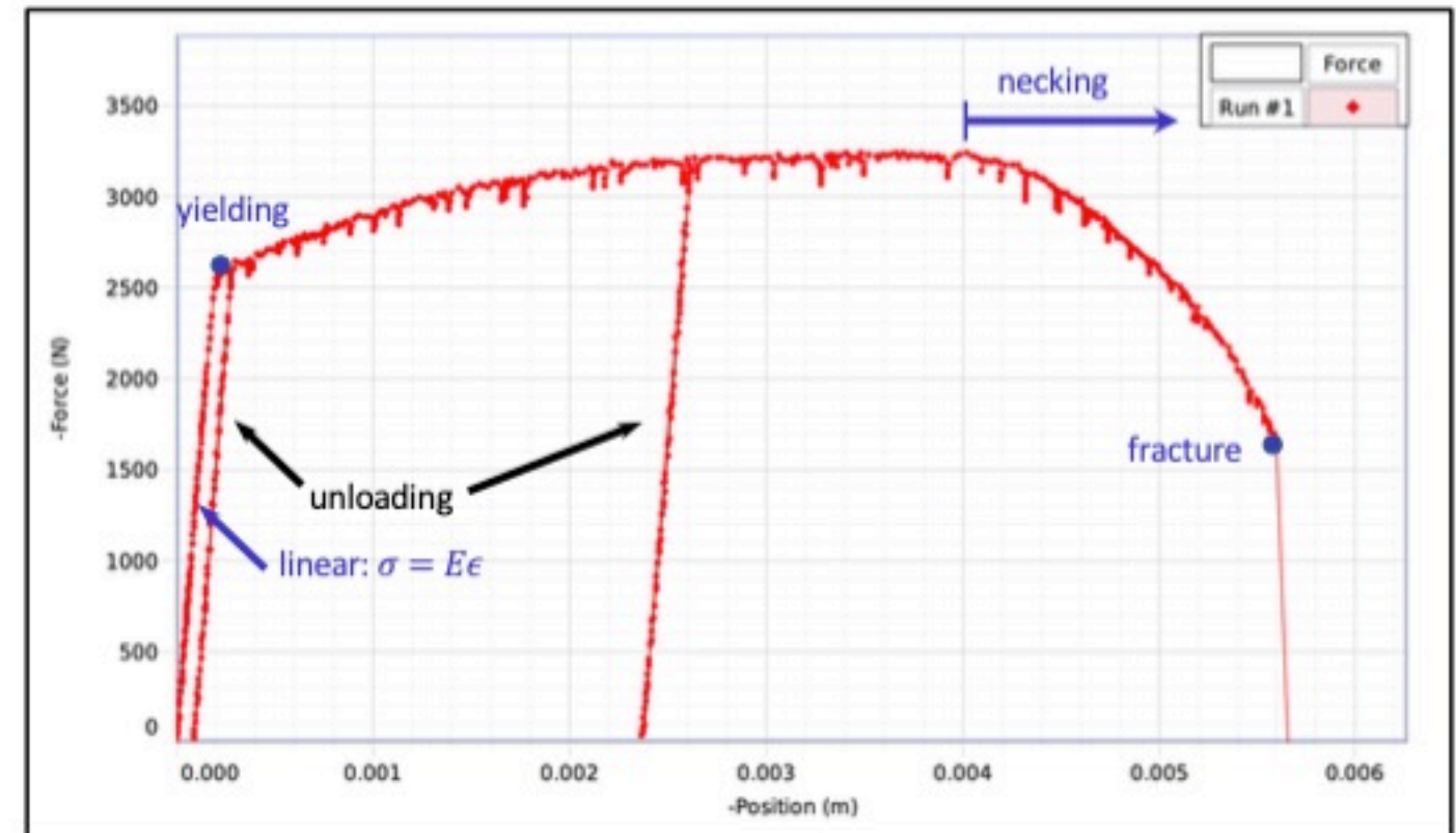
Load vs. elongation
