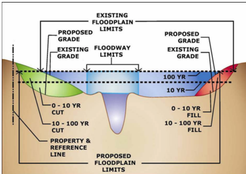
Figure 11-4 – Example Cross Section D-D
