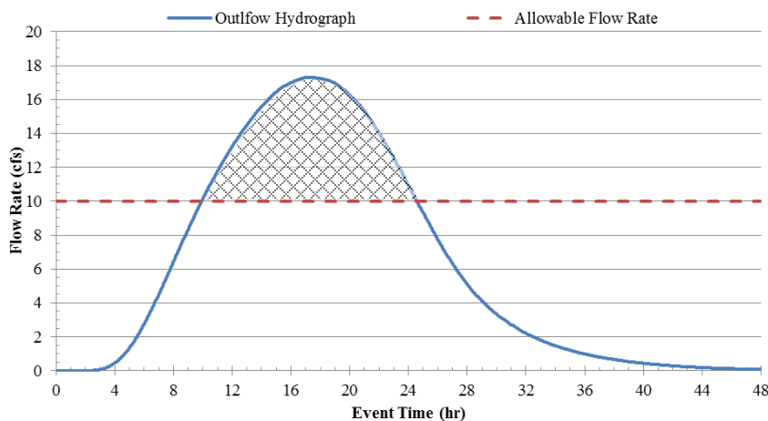
FIGURE 3-1 Required Storage Volume Determination Example
